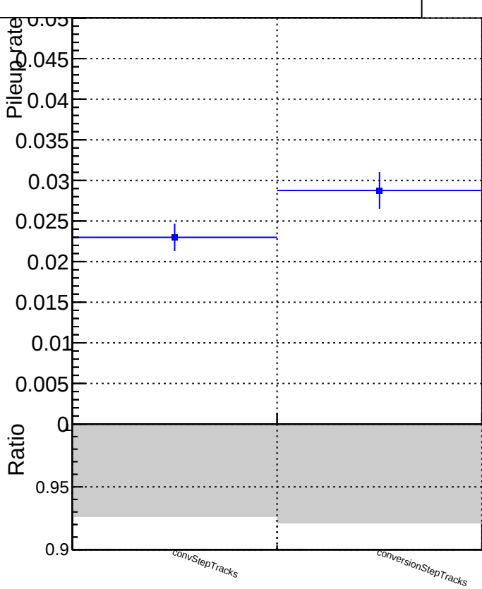
DQM_V0001_R000000001_Global_CMSSW_X_Y_Z_RECO
