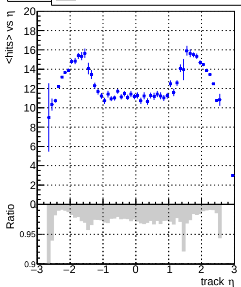
mean hits vs \eta DQM_V0001_R000000001_Global_CMSSW_X.Y.Z_RECO
