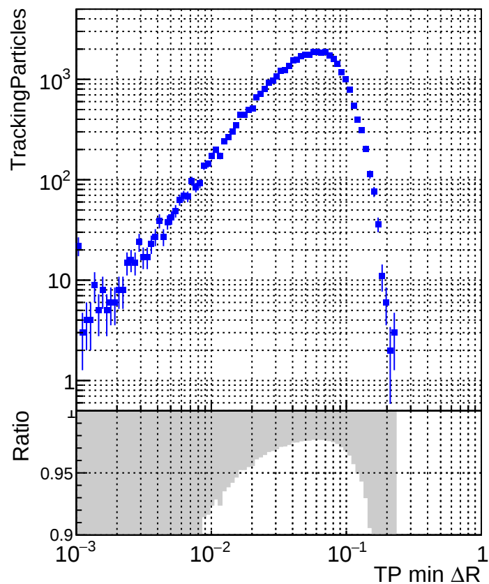
N of simulated tracks vs TP \Delta R (TP, jet) DQM_V0001_R000000001_Global_CMSSW_X_Y_Z_RECO
