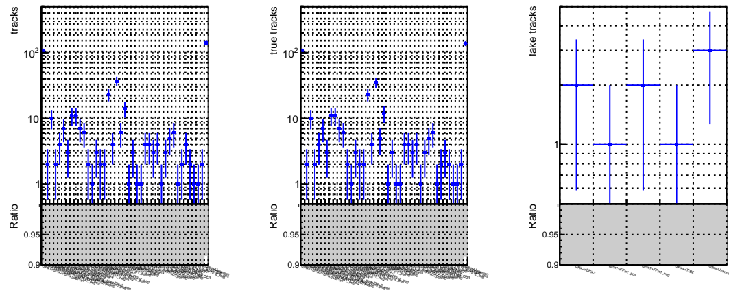
N of reco track vs. \chi^2 DQM_V0001_R000000001_Global_CMSSW_X_Y_Z_RECO
