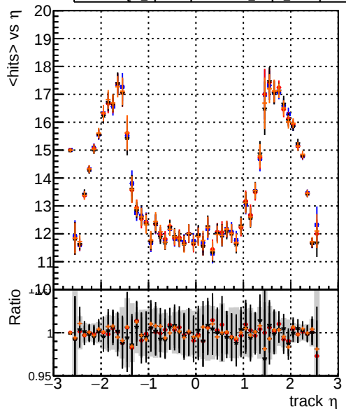
DQM_noIT_step2_ttbar-phase1-newgeom DQM_noCPE_step2_ttbar-phase1-newgeom DQM_cpeGenericTime_step2_ttbar-phase1-newgeom DQM_cpeTemplatedTime_step2_ttbar-phase1-newgeom
