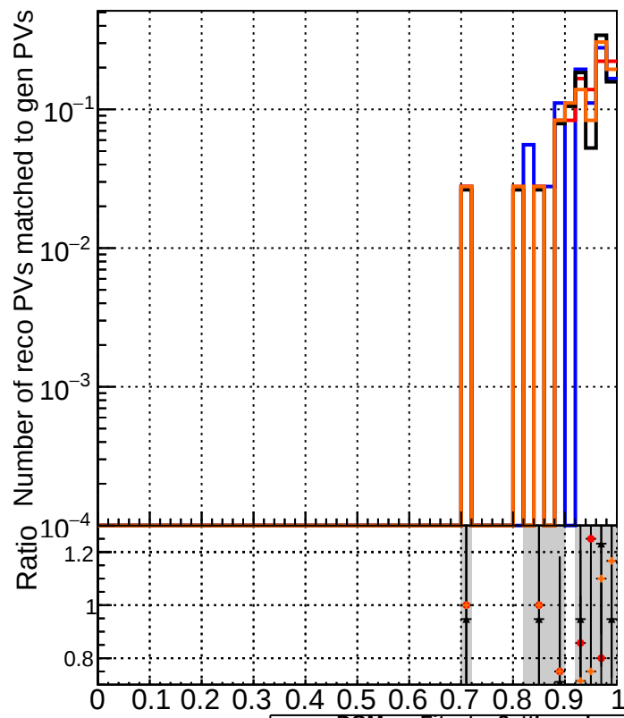
RecoPVAssoc2GenPVMatched_Purity
