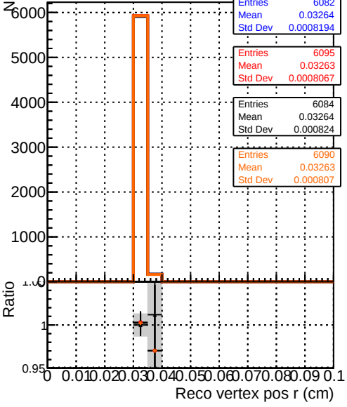
Recons Legend: - DQM_noFit_step2_ttbar-phase1-newgeom (blue line with circles) - DQM_noCPE_step2_ttbar-phase1-newgeom (red line with circles) - DQM_cpeGenericTime_step2_ttbar-phase1-newgeom (black line with circles) - DQM_cpeTemplatedTime_step2_ttbar-phase1-newgeom (orange line with circles)
