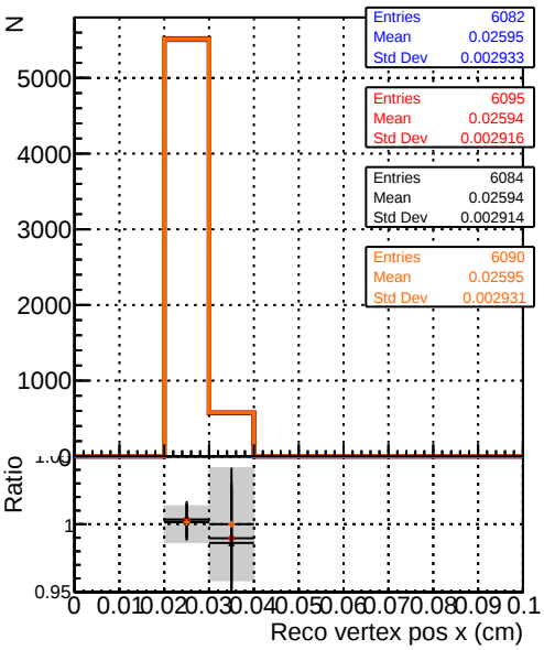
Recons Legend: - DQM_noFit_step2_ttbar-phase1-newgeom (blue line with circles) - DQM_noCPE_step2_ttbar-phase1-newgeom (red line with circles) - DQM_cpeGenericTime_step2_ttbar-phase1-newgeom (black line with circles) - DQM_cpeTemplatedTime_step2_ttbar-phase1-newgeom (orange line with circles)
