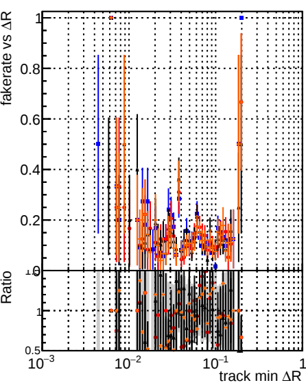
Fake rate vs \Delta R(\text{track, jet}) Legend: DOM noFit step2 ttbar-phase1-newgeom (blue) DOM noCP step2 ttbar-phase1-newgeom (red) DOM cpeGenericTime step2 ttbar-phase1-newgeom (black) DOM cpeTemplatedTime step2 ttbar-phase1-newgeom (orange)
