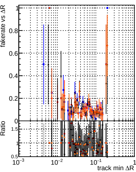
Fake rate vs \Delta R(\text{track, jet}) Legend: DOM noFit step2 tbar-phase1-newgeom DOM noCP step2 tbar-phase1-newgeom DOM cpe Generic time step2 tbar-phase1-newgeom DOM cpe+empl time step2 tbar-phase1-newgeom
