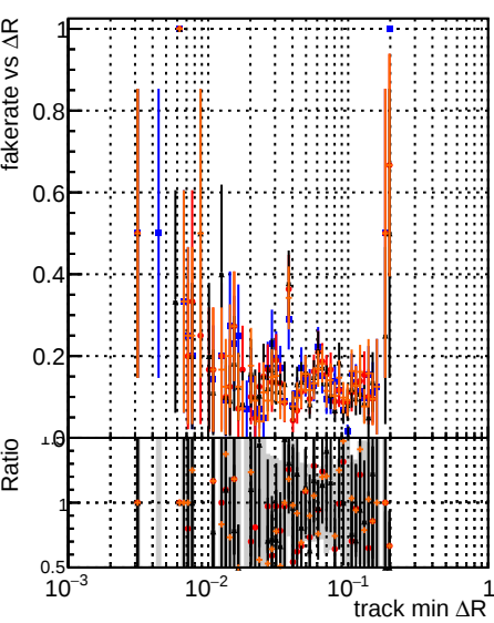
Fake rate vs \Delta R(\text{track, jet}) Legend: DQM noFit step2 ttbar-phase1-newgeom DQM noCP step2 ttbar-phase1-newgeom DQM noGenetic step2 ttbar-phase1-newgeom DQM cpe templated time step2 ttbar-phase1-newgeom
