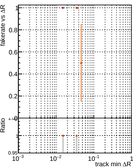
Fake rate vs \Delta R(\text{track, jet}) Legend: DOM noFit, step2, tbar-phase1, newgeom (blue) DOM noCP, step2, tbar-phase1, newgeom (red) DOM noCP, step2, tbar-phase1, newgeom (orange) DOM cpe, templated time, step2, tbar-phase1, newgeom (black)
