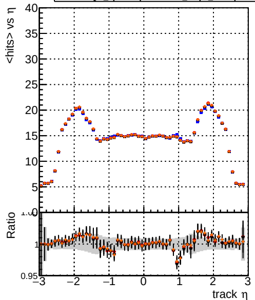
— DQM_noIt_step2_ttbar-phase1-newgeom — DQM_noCPE_step2_ttbar-phase1-newgeom — DQM_cpeGenericTime_step2_ttbar-phase1-newgeom — DQM_cpeTemplatedTime_step2_ttbar-phase1-newgeom mean hit
