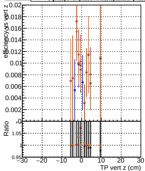
Efficiency vs TP vert z (cm) —•— DQM_noIt_step2_ttbar-phase1-newgeom —•— DQM_noCPE_step2_ttbar-phase1-newgeom —•— DQM_cpeGenericTime_step2_ttbar-phase1-newgeom —•— DQM_cpeTemplatedTime_step2_ttbar-phase1-newgeom
