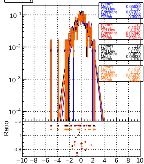
Legend: Blue line: BSM 100 GeV, \sqrt{s}=2 TeV, phase 1, \sqrt{s}=10 TeV, \sqrt{s}=100 TeV Red line: BSM 100 GeV, \sqrt{s}=2 TeV, phase 1, \sqrt{s}=10 TeV, \sqrt{s}=100 TeV Orange line: BSM 100 GeV, \sqrt{s}=2 TeV, phase 1, \sqrt{s}=10 TeV, \sqrt{s}=100 TeV
