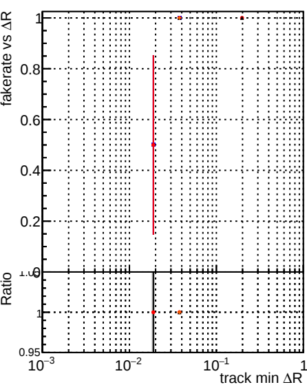
Fake rate vs \Delta R(\text{track, jet}) DQM noFit_step2_tbar-phase1-newgeom DQM noCP_step2_tbar-phase1-newgeom DQM noGenetic_step2_tbar-phase1-newgeom DQM cpeTemplatedTime_step2_tbar-phase1-newgeom
