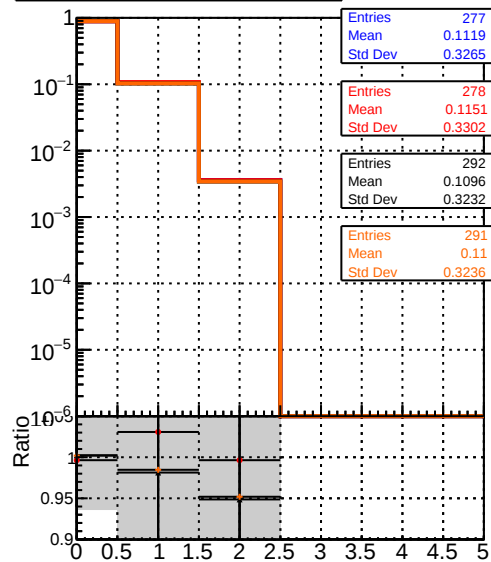
mean hit DQM_noFit_step2_ttbar-phase1-newgeom DQM_noCPE_step2_ttbar-phase1-newgeom DQM_cpeGenericTime_step2_ttbar-phase1-newgeom DQM_cpeTemplatedTime_step2_ttbar-phase1-newgeom
