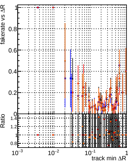
Fake rate vs \Delta R(\text{track, jet}) Legend: DOM noFit step2 tbar-phase1-newgeom (blue) DOM noCP step2 tbar-phase1-newgeom (red) DOM cpeGenericTime step2 tbar-phase1-newgeom (black) DOM cpeEmplantedTime step2 tbar-phase1-newgeom (orange)
