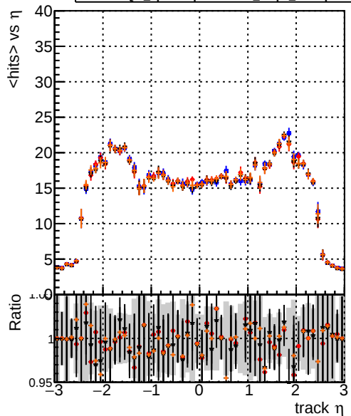
mean hits — DQM_noFit_step2_ttbar-phase1-newgeom — DQM_noCPE_step2_ttbar-phase1-newgeom — DQM_cpeGenericTime_step2_ttbar-phase1-newgeom — DQM_cpeTemplatedTime_step2_ttbar-phase1-newgeom
