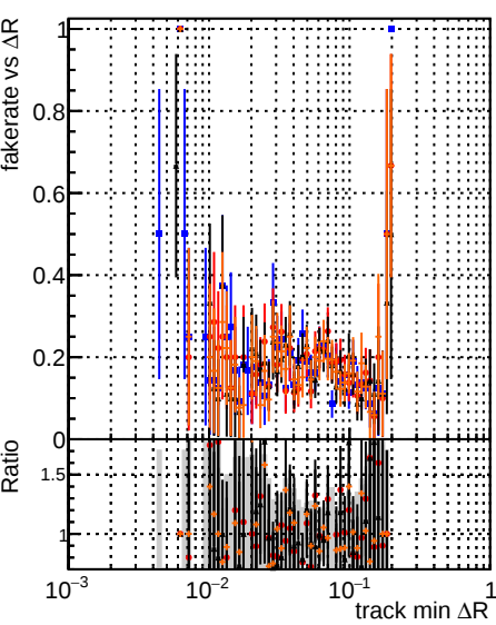
Fake rate vs \Delta R(\text{track, jet}) Legend: DQM noFit step2 ttbar-phase1-newgeom DQM noCP step2 ttbar-phase1-newgeom DQM noGen step2 ttbar-phase1-newgeom DQM cpe templated time step2 ttbar-phase1-newgeom
