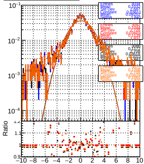
Legend: BDM (blue), BDM with 2nd order phase transition (red), BDM with time step and phase transition (orange)
