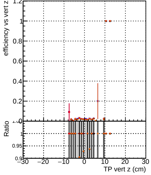
Efficiency vs vert z —●— DQM_noIt_step2_ttbar-phase1-newgeom —●— DQM_noCPE_step2_ttbar-phase1-newgeom —●— DQM_cpeGenericTime_step2_ttbar-phase1-newgeom —●— DQM_cpeTemplatedTime_step2_ttbar-phase1-newgeom
