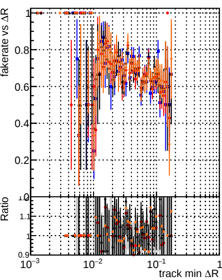
Fake rate vs \Delta R(\text{track, jet}) Legend: DQM noFit step2 tbar-phase1-newgeom (blue) DQM noCP step2 tbar-phase1-newgeom (red) DQM noGen step2 tbar-phase1-newgeom (black) DQM cpe templated time step2 tbar-phase1-newgeom (orange)
