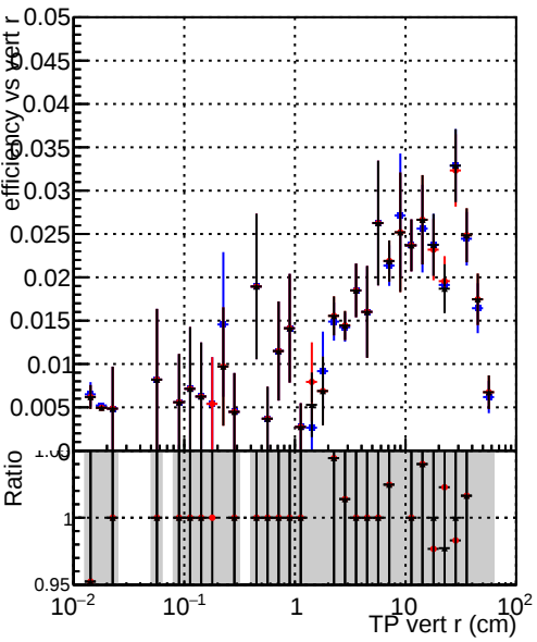
Efficiency vs vertpos DQM_original_step2_ttbar-phase1-newgeom DQM_mkFit_step2_ttbar-phase1-newgeom DQM_pixelCPETemplate_step2_ttbar-phase1-newgeom
