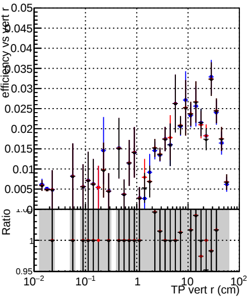
Efficiency vs vertpos Legend: DQM_original_step2_ttbar-phase1-newgeom DQM_mkFit_step2_ttbar-phase1-newgeom DQM_pixelCPETemplate_step2_ttbar-phase1-newgeom
