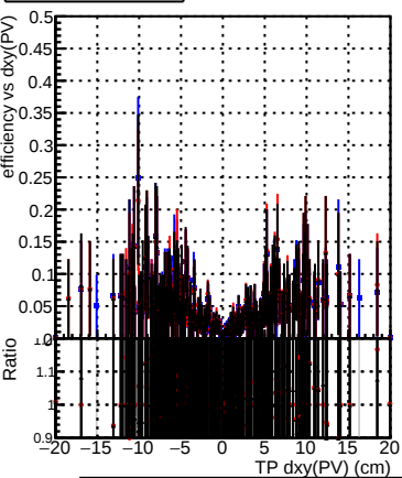
Efficiency vs Dxy(PV) Legend: DQM_original_step2_ttbar-phase1-newgeom DQM_mkFit_step2_ttbar-phase1-newgeom DQM_pixelCPETemplate_step2_ttbar-phase1-newgeom
