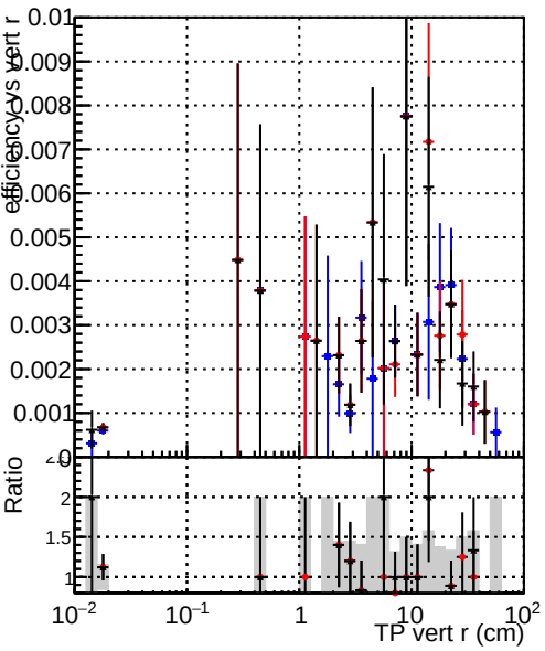
Efficiency vs TP vert r (cm) Legend: DQM_original_step2_ttbar-phase1-newgeom DQM_mkFit_step2_ttbar-phase1-newgeom DQM_pixelCPETemplate_step2_ttbar-phase1-newgeom
