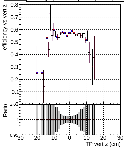
Efficiency vs. TP vert z (cm) —●— DQM_original_step2_ttbbar-phase1-newgeom —●— DQM_mkFit_step2_ttbbar-phase1-newgeom —●— DQM_pixelCPETemplate_step2_ttbbar-phase1-newgeom
