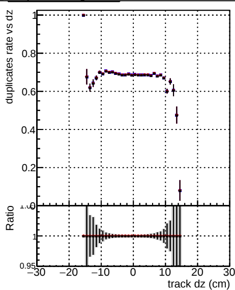
DOM original_step2_tbar-phase1-newgeom DOM mkFit_step2_tbar-phase1-newgeom DOM pixelCPEtemplate_step2_tbar-phase1-newgeom
