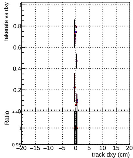
DOM original_step2_tbar-phase1-newgeom DOM mkFit_step2_tbar-phase1-newgeom DOM pixelCPEtemplate_step2_tbar-phase1-newgeom
