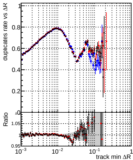
—■— DQM_original_step2_ttbbar-phase1-newgeom —●— DQM_mkFit_step2_ttbbar-phase1-newgeom —×— DQM_pixelCPETemplate_step2_ttbbar-phase1-newgeom
