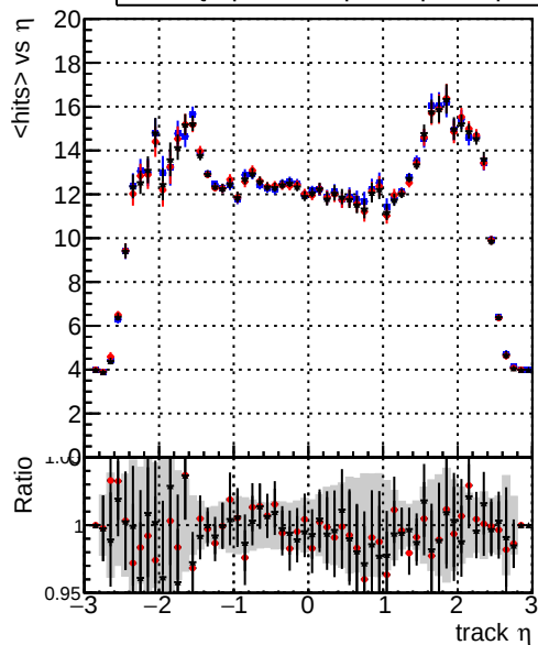
mean hit — DQM_original_step2_ttbbar-phase1-newgeom — DQM_mkFit_step2_ttbbar-phase1-newgeom — DQM_pixelCPETemplate_step2_ttbbar-phase1-newgeom
