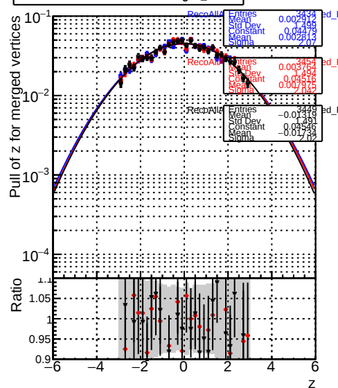
RecoAllAssoc2GenMatchedMerged_PullZ
