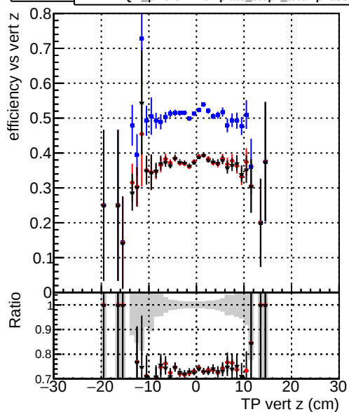
Efficiency vs. TP vert z (cm) — DQM_original_step2_ttbarm-phase1-newgeom — DQM_mkFit_step2_ttbarm-phase1-newgeom — DQM_pixelCPETemplate_step2_ttbarm-phase1-newgeom
