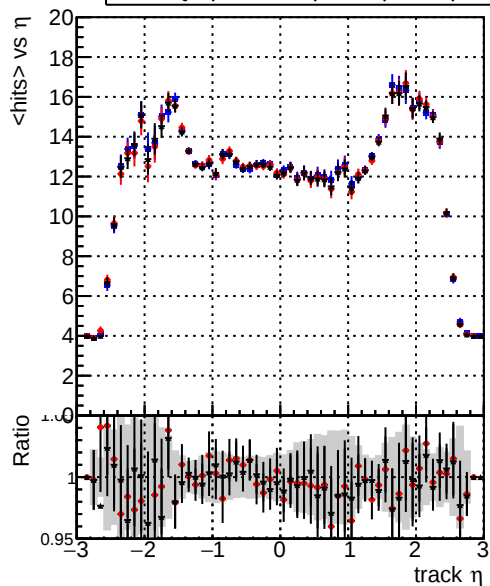
mean hits — DQM_original_step2_ttbbar-phase1-newgeom — DQM_mkFit_step2_ttbbar-phase1-newgeom — DQM_pixelCPETemplate_step2_ttbbar-phase1-newgeom
