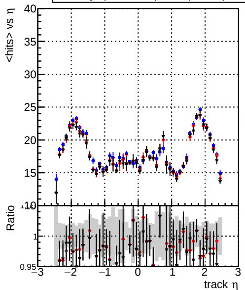
— DQM_original_step2_ttbar-phase1-newgeom — DQM_mkFit_step2_ttbar-phase1-newgeom — DQM_pixelCPEtemplate_step2_ttbar-phase1-newgeom mean hits
