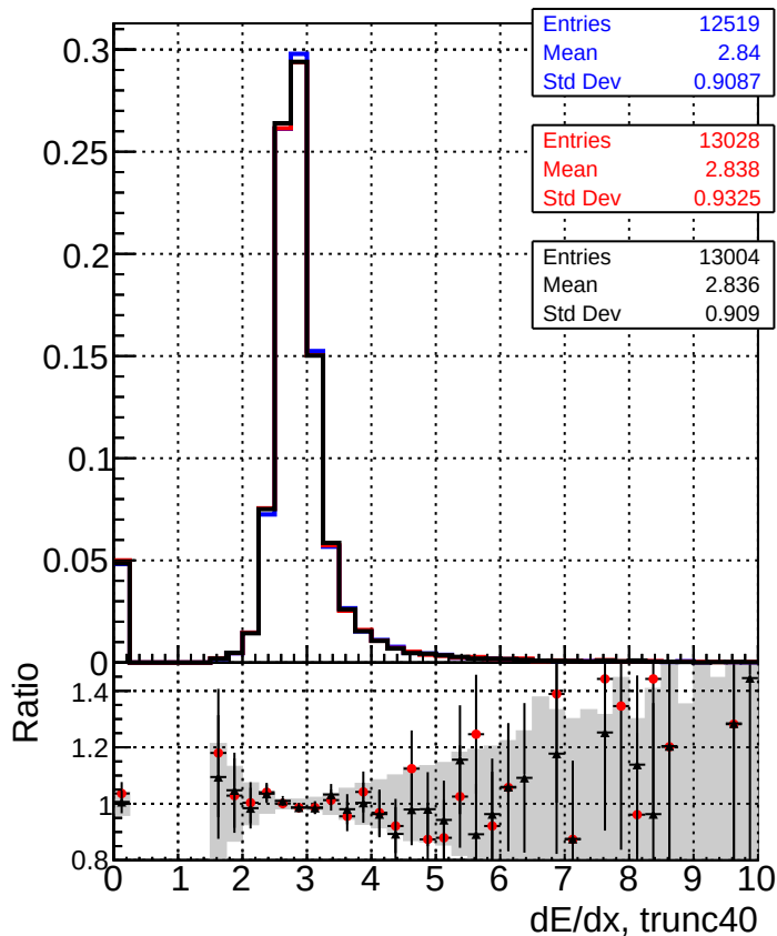
— DQM_original_step2_ttbar-phase1-newgeom — DQM_mkFit_step2_ttbar-phase1-newgeom — DQM_pixelCPETemplate_step2_ttbar-phase1-newgeom
