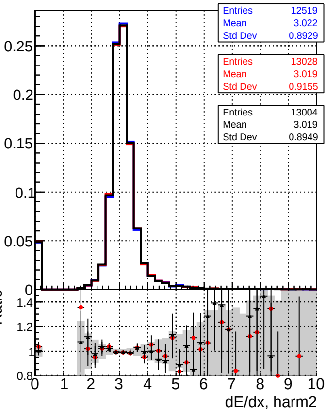
— DQM_original_step2_ttbar-phase1-newgeom — DQM_mkFit_step2_ttbar-phase1-newgeom — DQM_pixelCPETemplate_step2_ttbar-phase1-newgeom
