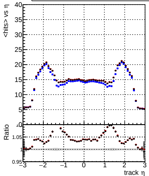
mean hits vs \eta — DQM_original_step2_ttbbar-phase1-newgeom — DQM_mkFit_step2_ttbbar-phase1-newgeom — DQM_pixelCPETemplate_step2_ttbbar-phase1-newgeom
