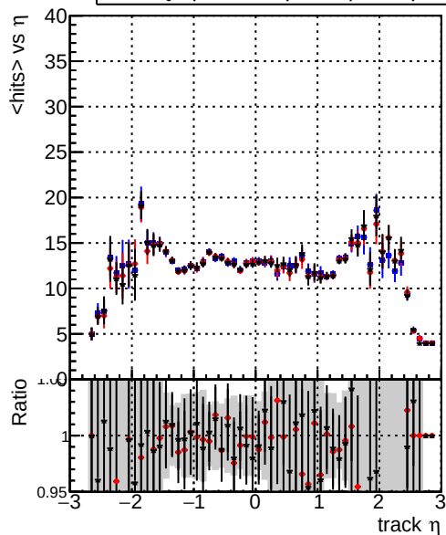
mean hits vs \eta — DQM_original_step2_ttbar-phase1-newgeom — DQM_mkFit_step2_ttbar-phase1-newgeom — DQM_pixelCPETemplate_step2_ttbar-phase1-newgeom
