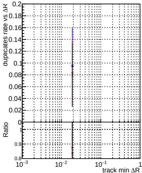
— DQM original step2 ttbar-phase1-newgeom — DQM mkFit step2 ttbar-phase1-newgeom — DQM pixelCPETemplate step2 ttbar-phase1-newgeom
