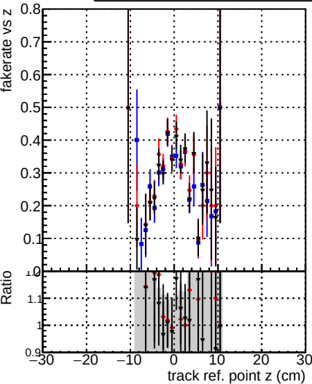
Fake rate vs verpos — DQM_original_step2_ttbar-phase1-newgeom — DQM_mkFit_step2_ttbar-phase1-newgeom — DQM_pixelCPETemplate_step2_ttbar-phase1-newgeom
