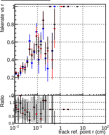
Fake rate vs verpos — DQM_original_step2_ttbar-phase1-newgeom — DQM_mkFit_step2_ttbar-phase1-newgeom — DQM_pixelCPETemplate_step2_ttbar-phase1-newgeom
