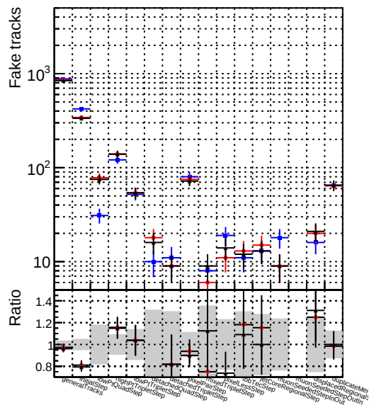
Number of tracks vs collection DQM_original_step2_ttbar-phase1-newgeom DQM_mkFit_step2_ttbar-phase1-newgeom DQM_pixelCPETemplate_step2_ttbar-phase1-newgeom
