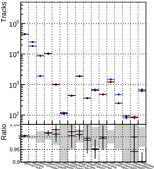
Number DQM_original_step2_ttbar-phase1-newgeom DQM_mkFit_step2_ttbar-phase1-newgeom DQM_pixelCPETemplate_step2_ttbar-phase1-newgeom
