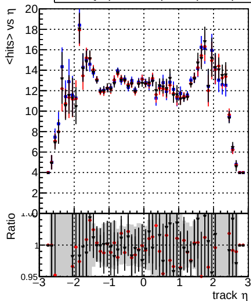
mean hit — DQM_original_step2_ttbar-phase1-newgeom — DQM_mkFit_step2_ttbar-phase1-newgeom — DQM_pixelCPETemplate_step2_ttbar-phase1-newgeom
