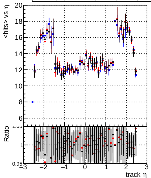
mean hit DQM_original_step2_ttbar-phase1-newgeom DQM_mkFit_step2_ttbar-phase1-newgeom DQM_pixelCPETemplate_step2_ttbar-phase1-newgeom
