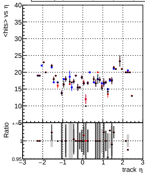
mean hit — DQM_original_step2_ttbbar-phase1-newgeom — DQM_mkFit_step2_ttbbar-phase1-newgeom — DQM_pixelCPETemplate_step2_ttbbar-phase1-newgeom
