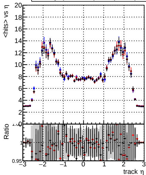
mean hit — DQM_original_step2_ttbar-phase1-newgeom — DQM_mkFit_step2_ttbar-phase1-newgeom — DQM_pixelCPETemplate_step2_ttbar-phase1-newgeom
