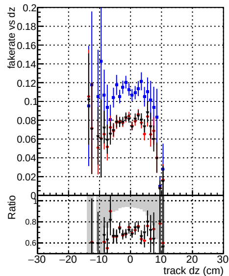
Fake rate vs dz Legend: DOM original_step2_tbar-phase1-newgeom DOM mk_fit_step2_tbar-phase1-newgeom DOM pixelCPE-template_step2_tbar-phase1-newgeom
