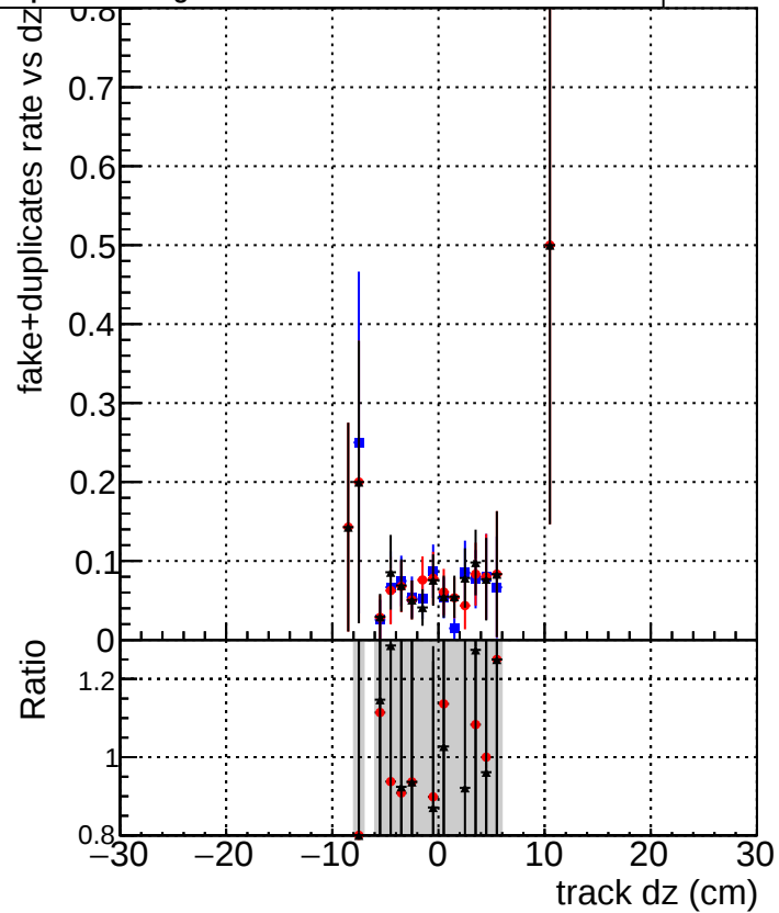
DQM_original_step2_ttbbar-phase1-newgeom DQM_mkFit_step2_ttbbar-phase1-newgeom DQM_pixelCPETemplate_step2_ttbbar-phase1-newgeom
