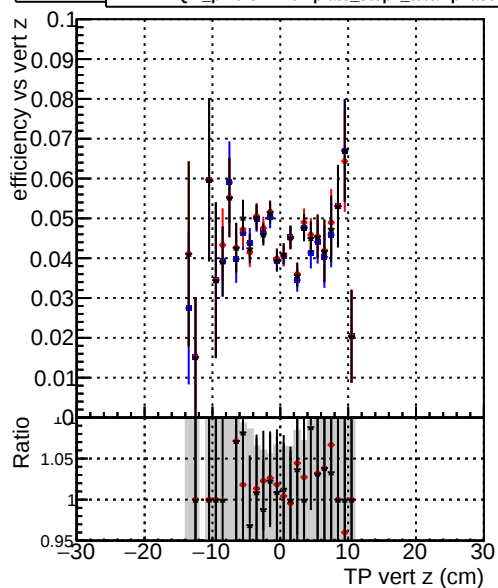
Efficiency vs vert z —●— DQM_original_step2_ttbbar-phase1-newgeom —●— DQM_mkFit_step2_ttbbar-phase1-newgeom —●— DQM_pixelCPETemplate_step2_ttbbar-phase1-newgeom
