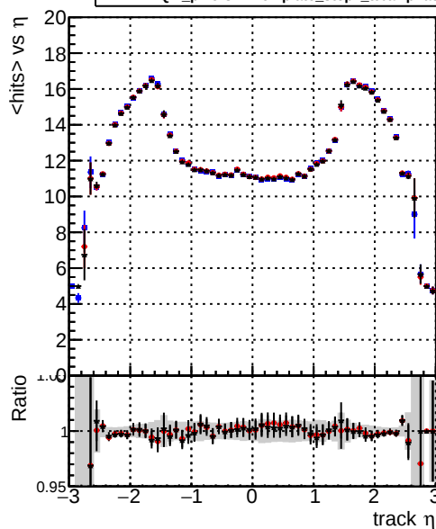
mean hits — DQM_original_step2_ttbar-phase1-newgeom — DQM_mkFit_step2_ttbar-phase1-newgeom — DQM_pixelCPETemplate_step2_ttbar-phase1-newgeom
