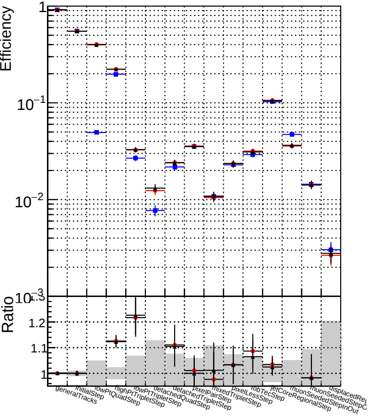
DQM_original_step2_ttbar-phase1-newgeom DQM_mkFit_step2_ttbar-phase1-newgeom DQM_pixelICPETemplate_step2_ttbar-phase1-newgeom
